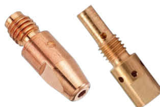
MIG WELDING TIP | MIG WELDING TIP HOLDER M6 0.8 X 6MM | 1.0 X 6MM | 0.8 X 8MM | 1.0 X 8MM
